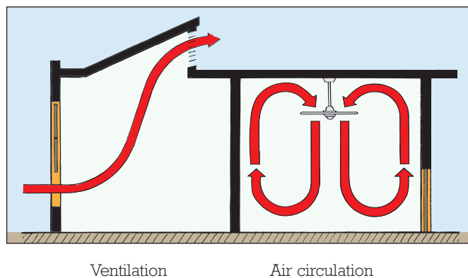
Figure 3.3 Create natural air flow for ventilation by having openings on opposite sides of rooms
