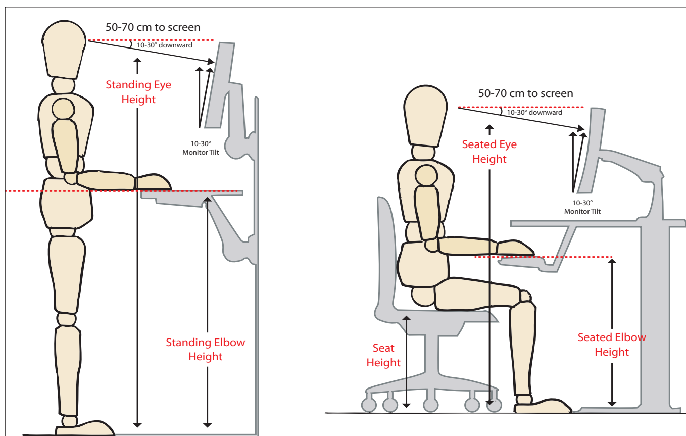
Figure 2.3 Recommended dimension for standing and seated tasks
