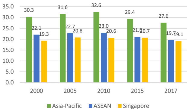
► Figure 9. Air quality PM 2.5 emissions, 2000-2017, Singapore, ASEAN and Asia-Pacific (micrograms per cubic metre)
