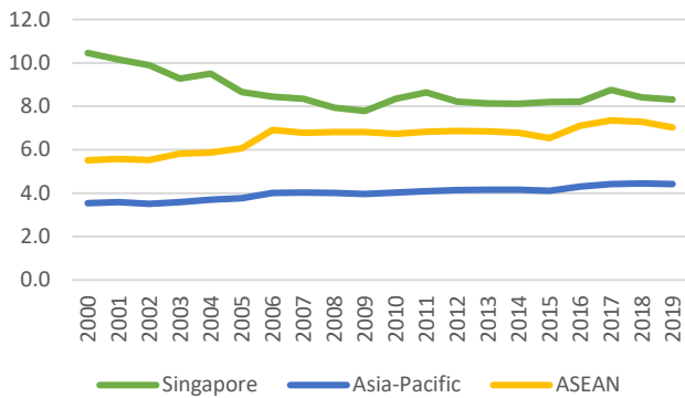
► Figure 8. CO2 emissions, 2000-2019, Singapore, ASEAN and Asia-Pacific (metric tonnes per capita)
