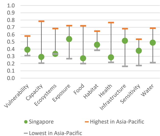
► Figure 10. Notre Dame Global Adaptation Index, Vulnerability and composite indicators, 2020, Singapore, Asia-Pacific (index score)
