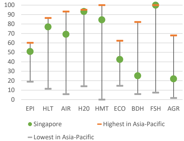
► Figure 5. Environmental performance index and selected indicators, Singapore and Asia-Pacific, 2022
